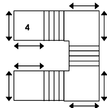
3 straight flights
